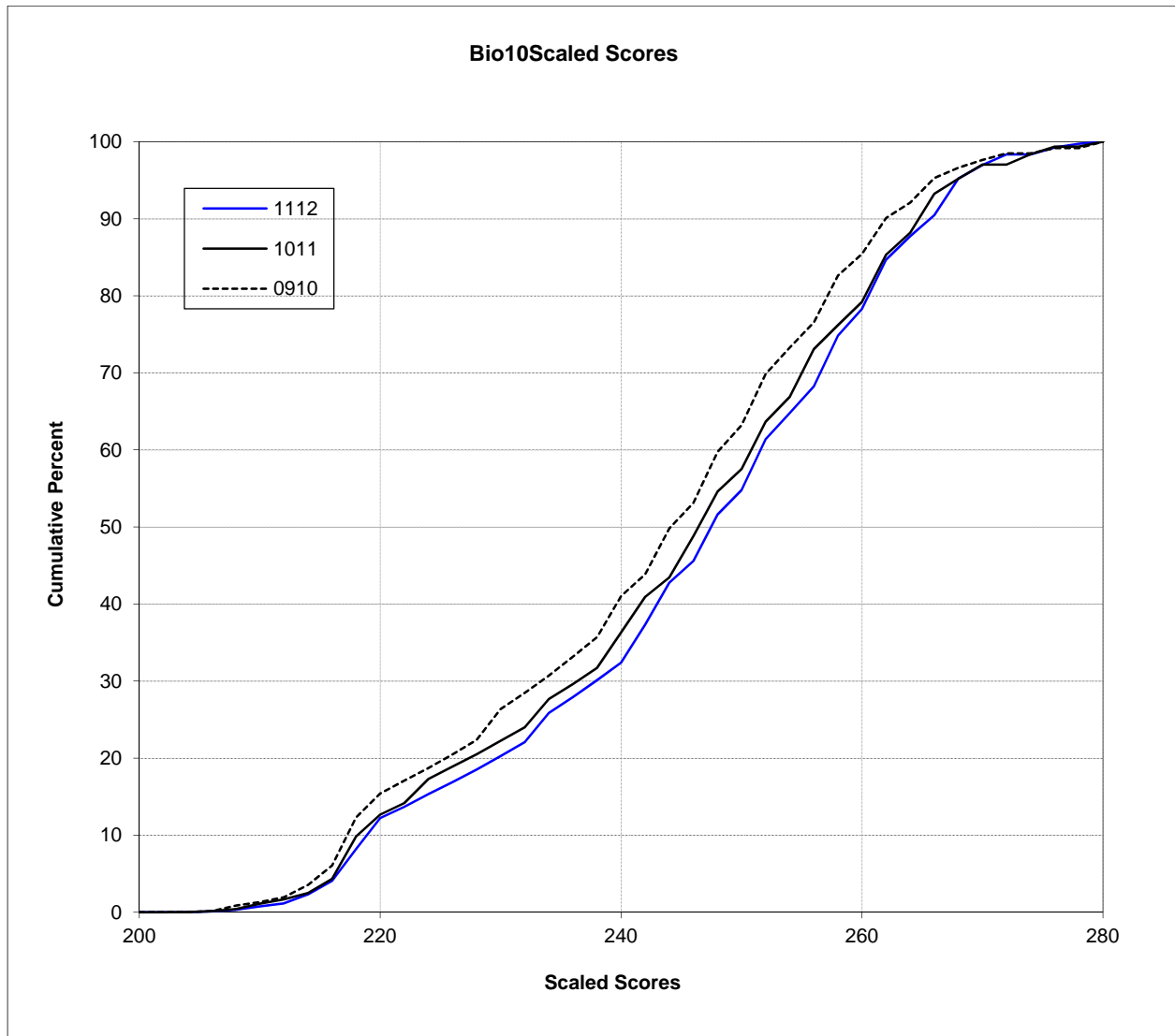
Figure N-17. 2012 MCAS: Cumulative Distribution Plot – High School Biology
