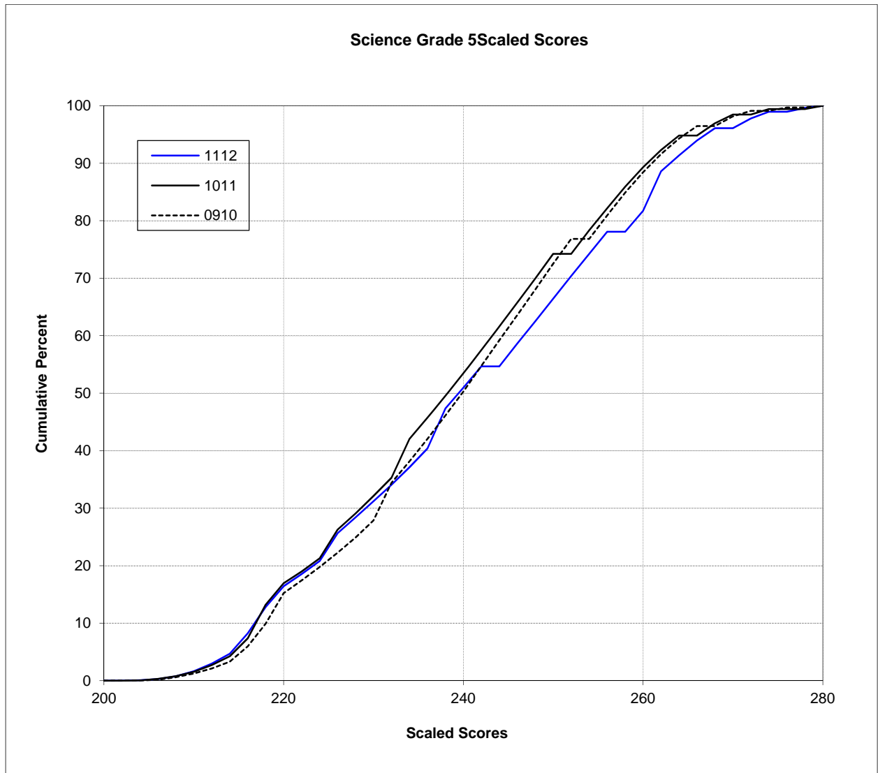
Figure N-15. 2012 MCAS: Cumulative Distribution Plot – STE Grade 5
