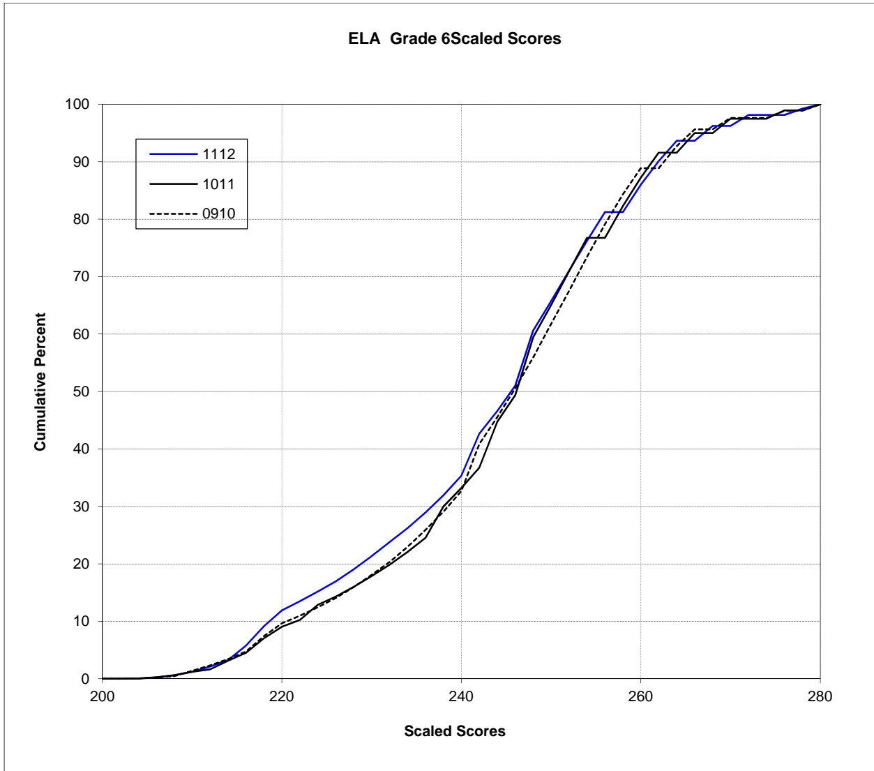
Figure N-4. 2012 MCAS: Cumulative Distribution Plot – ELA Grade 6
