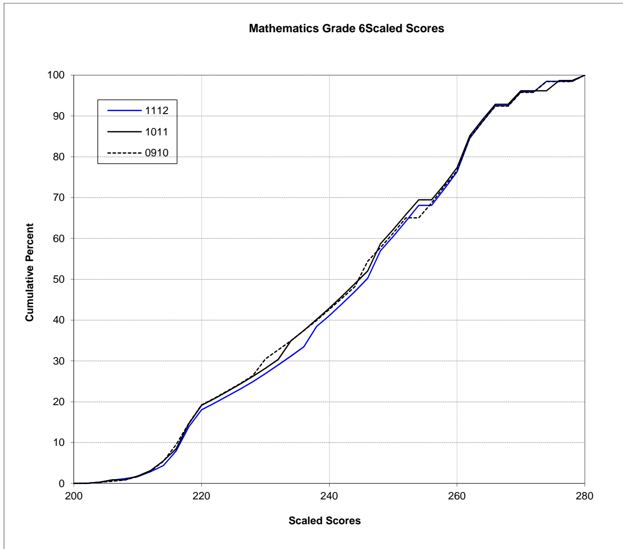
Figure N-11. 2012 MCAS: Cumulative Distribution Plot – Mathematics Grade 6
