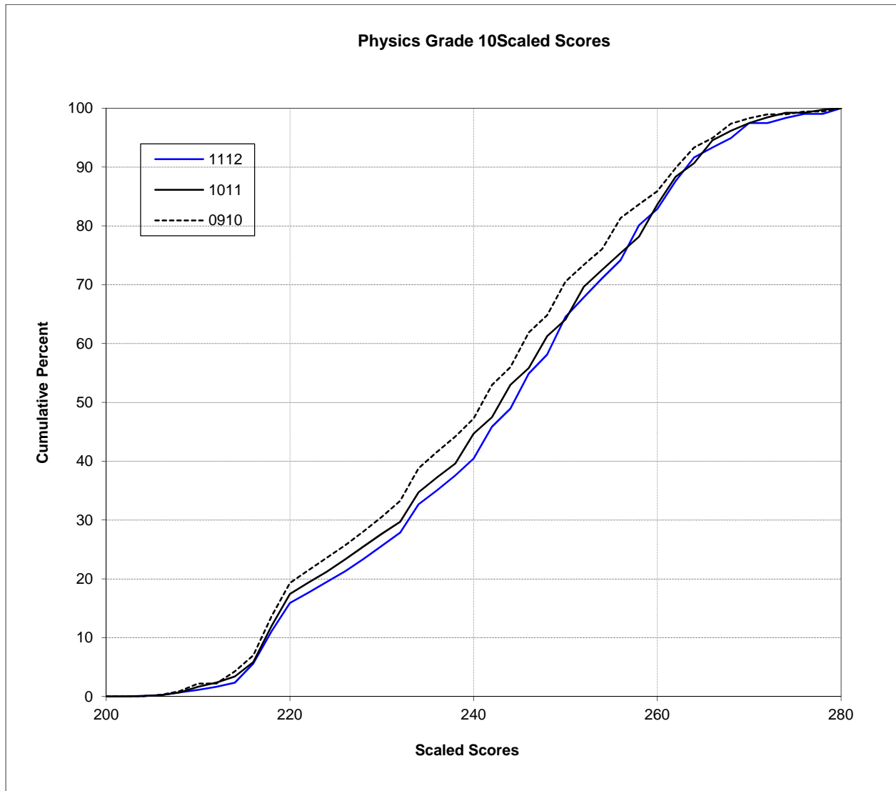
Figure N-19. 2012 MCAS: Cumulative Distribution Plot – High School Introductory Physics
