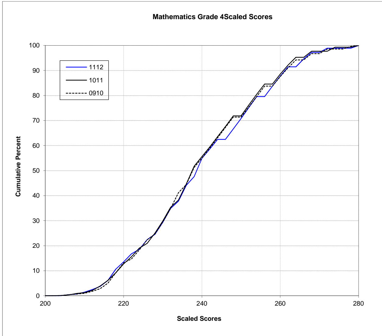
Figure N-9. 2012 MCAS: Cumulative Distribution Plot – Mathematics Grade 4
