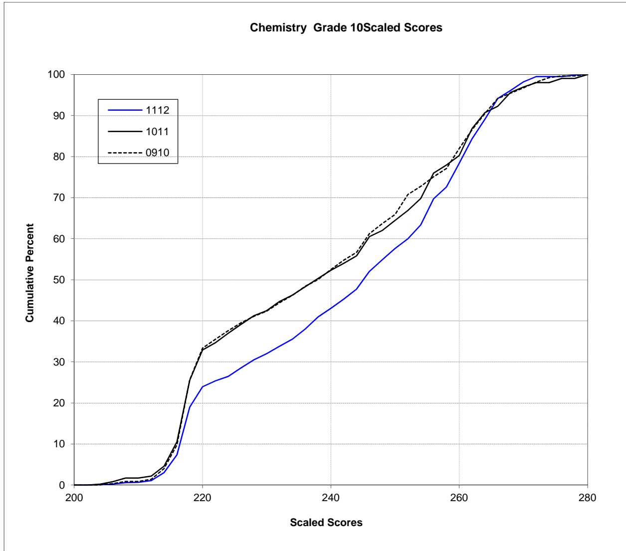
Figure N-18. 2012 MCAS: Cumulative Distribution Plot – High School Chemistry
