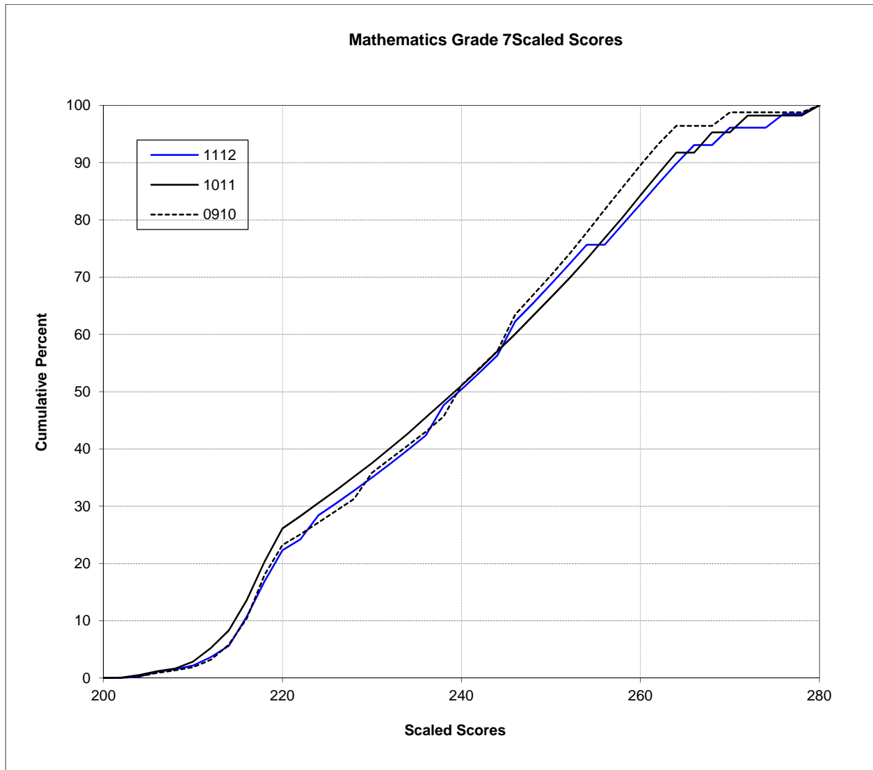
Figure N-12. 2012 MCAS: Cumulative Distribution Plot – Mathematics Grade 7
