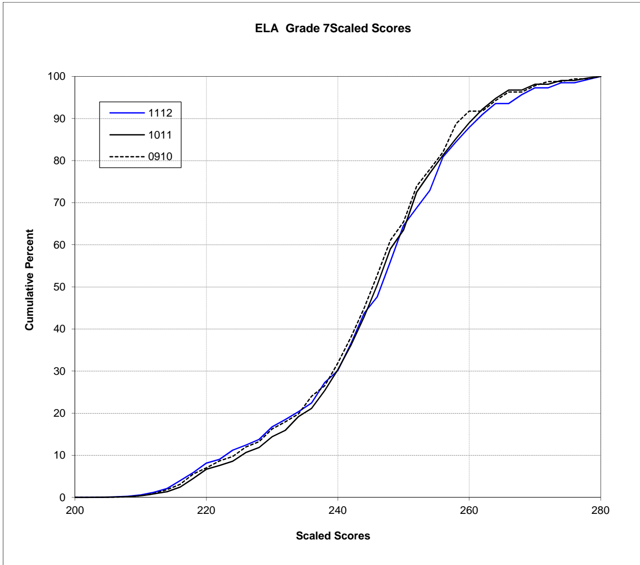
Figure N-5. 2012 MCAS: Cumulative Distribution Plot – ELA Grade 7
