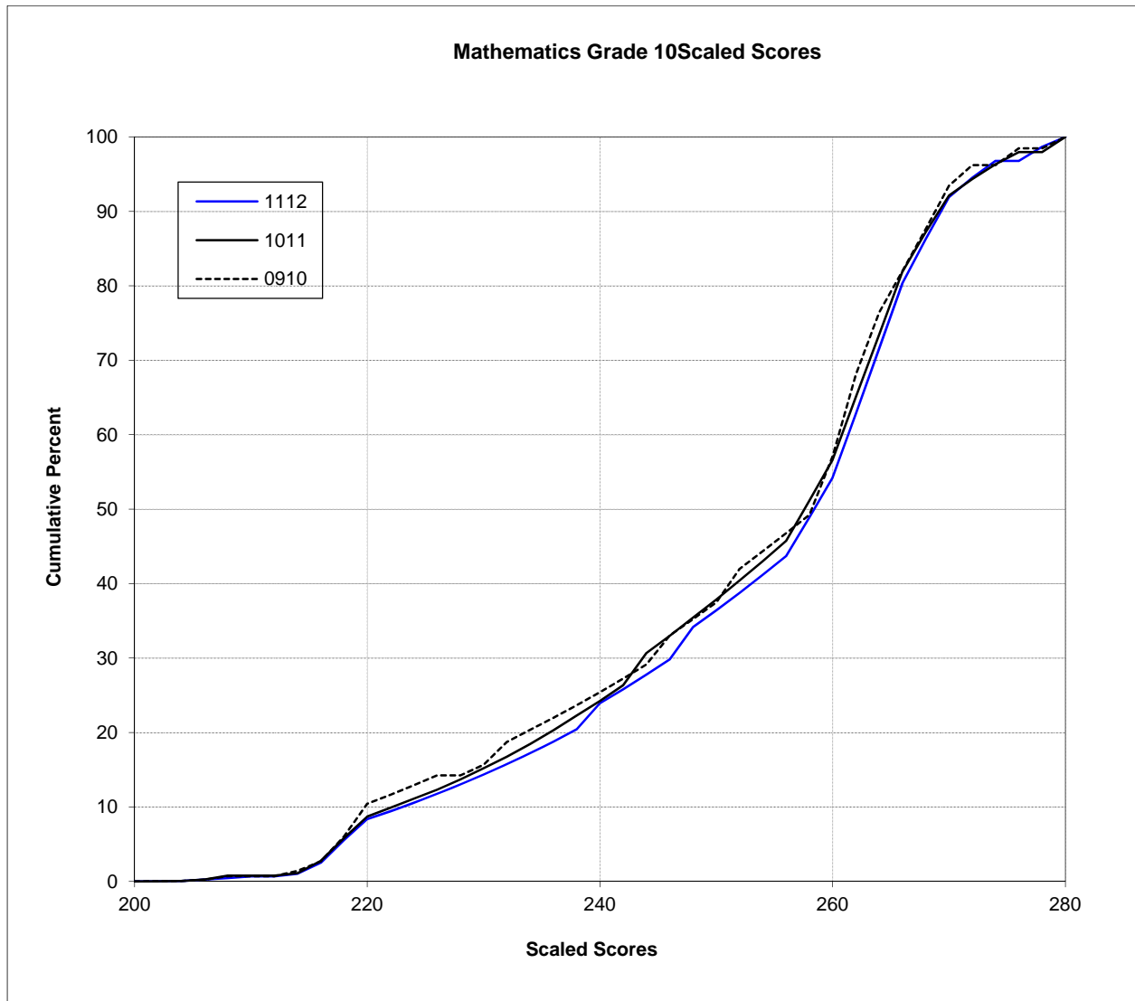
Figure N-14. 2012 MCAS: Cumulative Distribution Plot – Mathematics Grade 10
